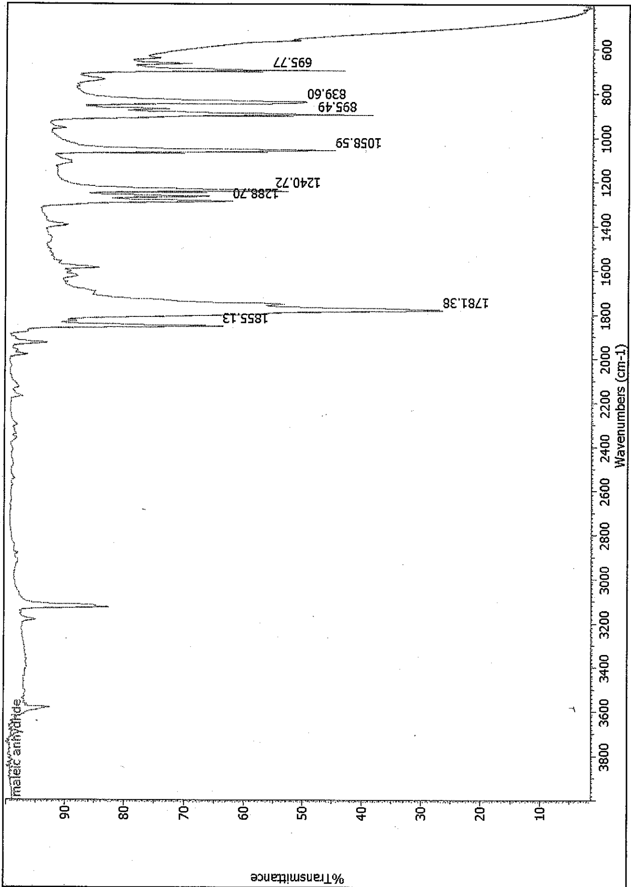
IR spectrum of maleic anhydride (thin film)
