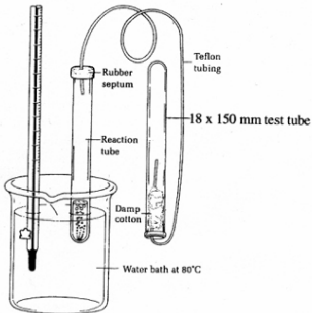
Reaction apparatus set-up with gas trap
