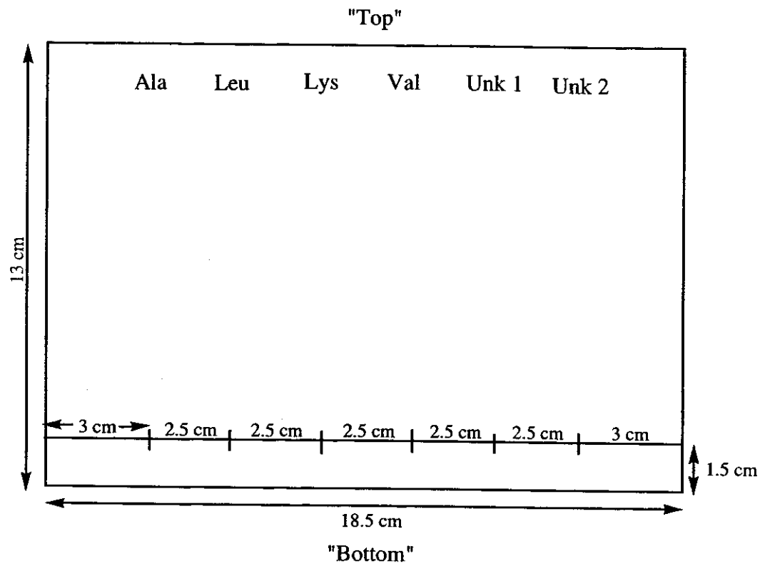
Figure 1. Dimensions and labeling for paper chromatography of amino acids
