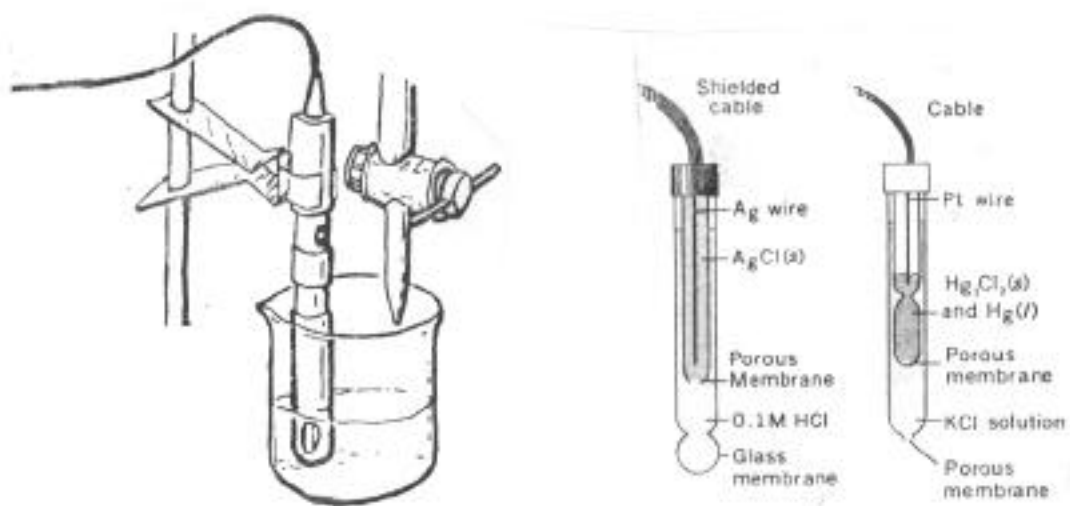
Titration apparatus set-up; glass electrode and calomel electrode.
