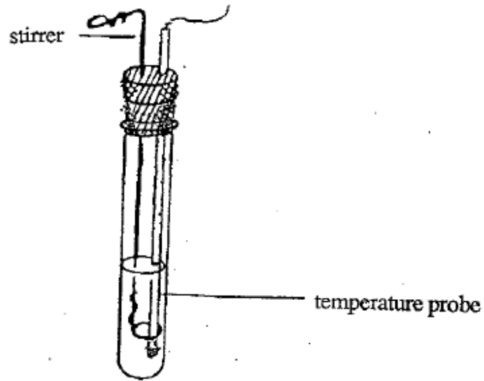
Figure 2. Set-up for determining freezing point depression.
