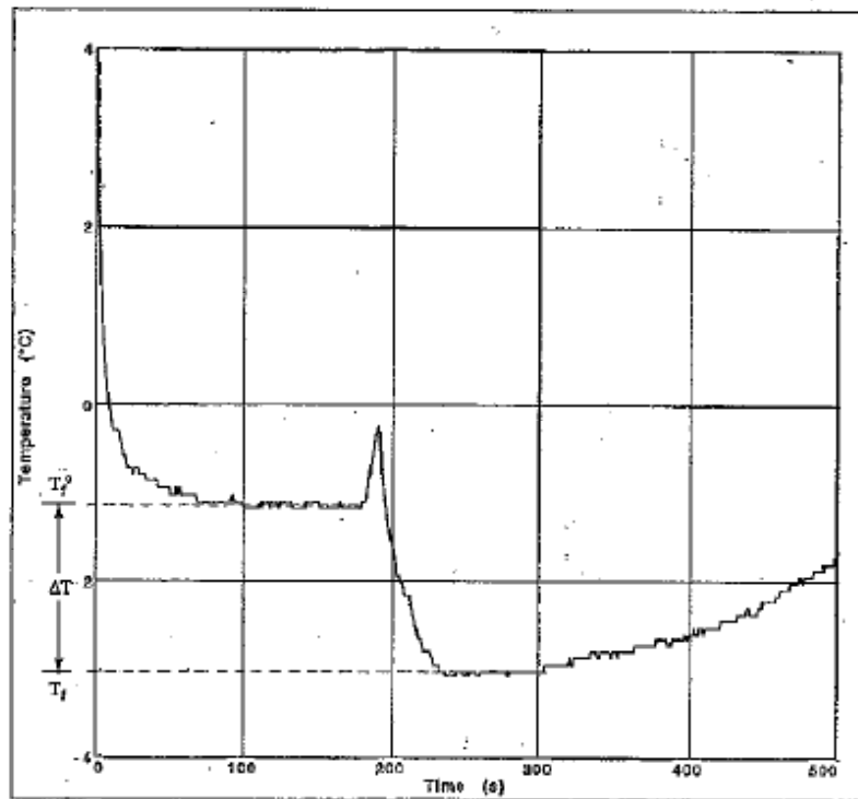
Figure 3. Plot of temperature as a function of time when a solute is added to an ice-water mixture.
