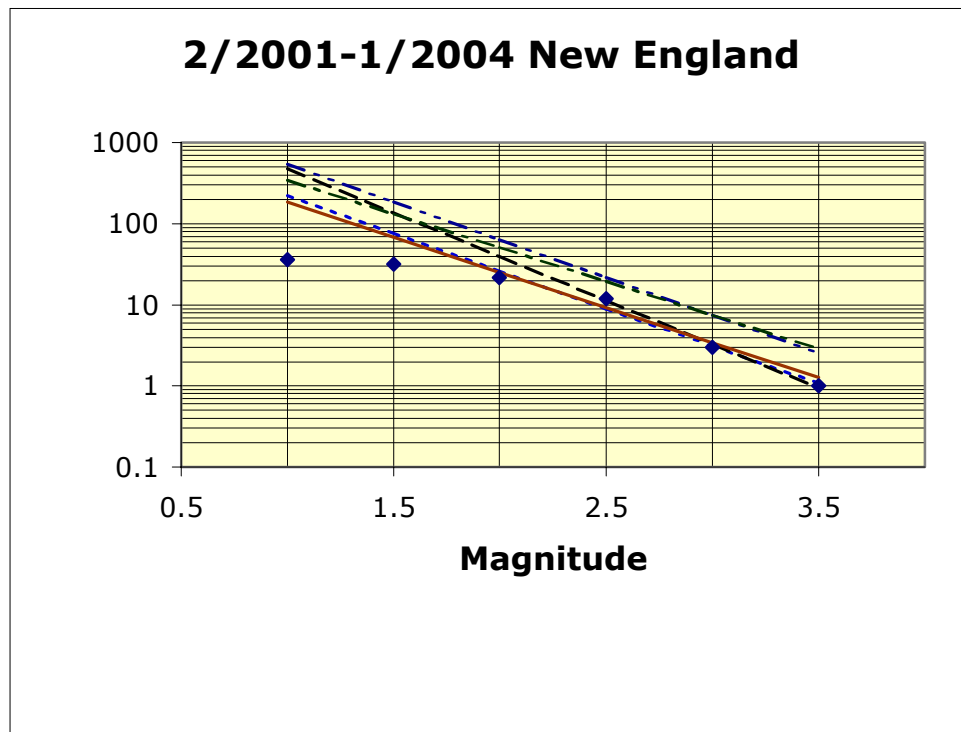
Figure 3. Gutenberg-Richter recurrence data for New England earthquakes from February 2001 through January 2004. Regression lines through the data points from magnitude 2.0 to 3.5, 2.5 to 3.5 and 2.0 to 3.0 are shown, as are recurrence curves for a three-year time period from Ebel (1987) from NEUS data from 1938 to 1986 and 1975 to 1986. For the Ebel (1987) recurrence curves, it was assumed that New England has half the spatial area of the entire northeastern U.S.
